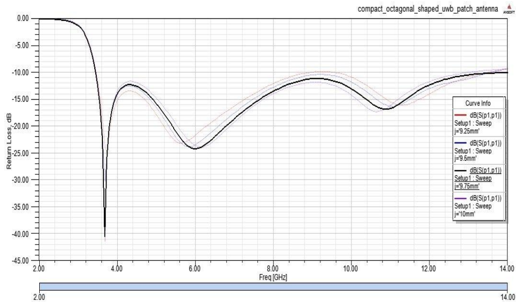
Fig. 3. Effects of varying slot width W_2
