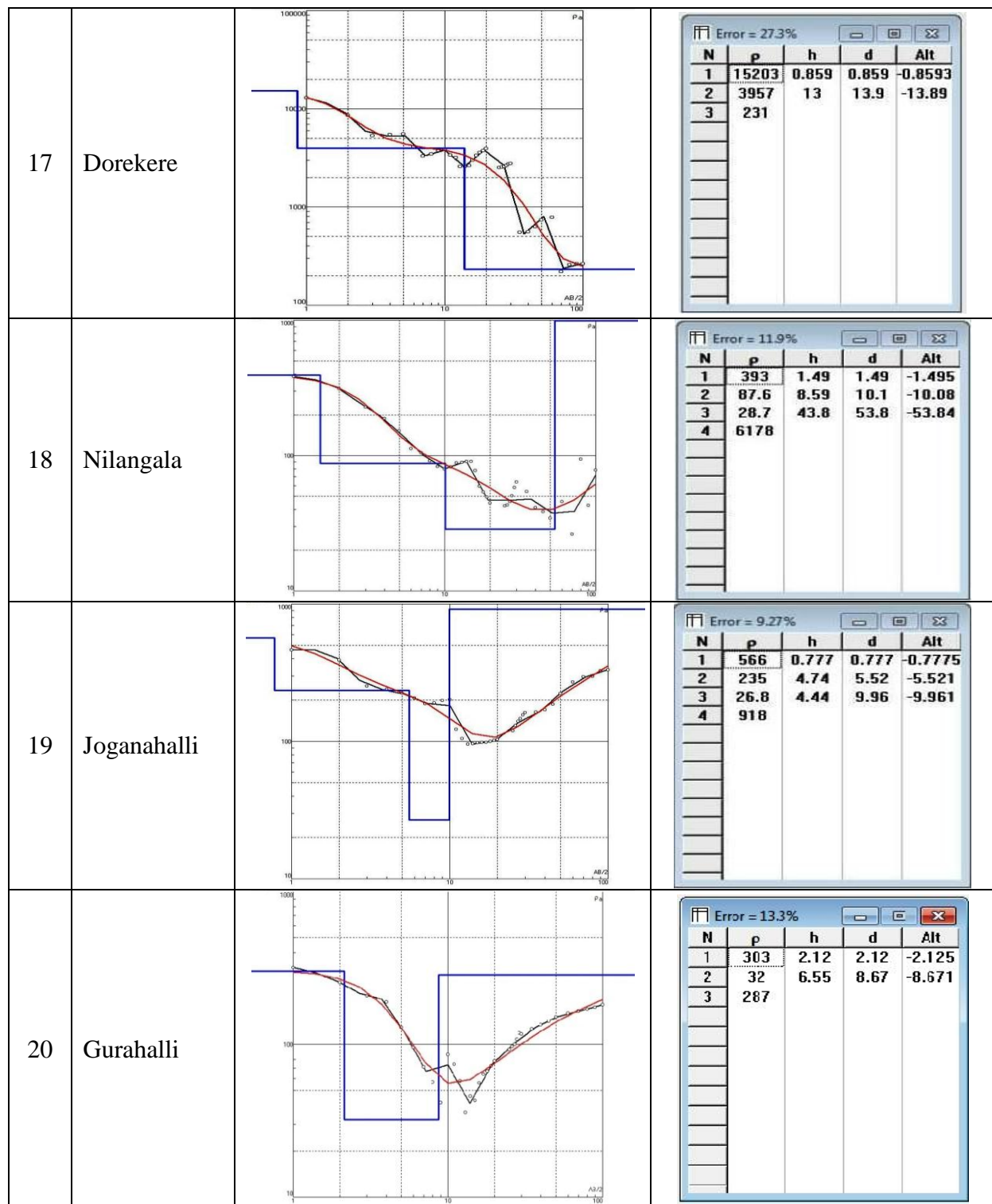
Fig. 6: Automated Fit of Ves Curves in Periyapatna Taluk.
