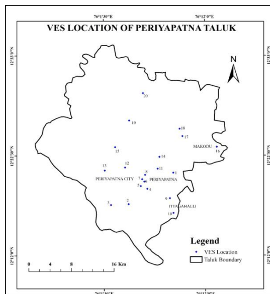
Fig. 3: VES location of the study area.
