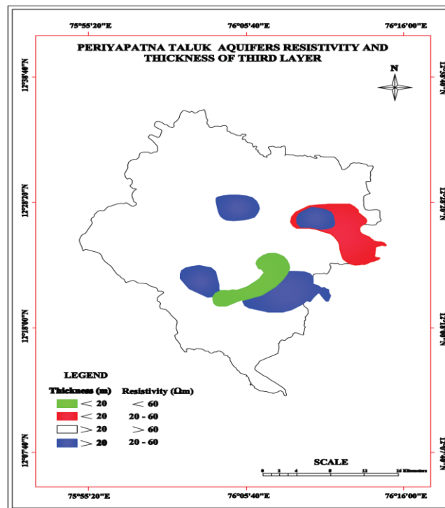
Fig. 7.7: Aquifers resistivity and thickness of Third Layer.
