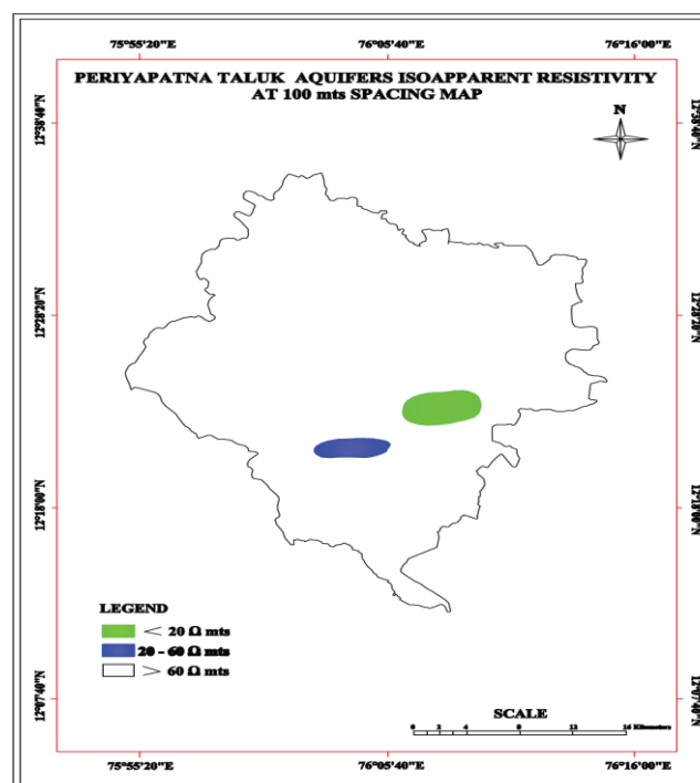
Fig. 7.4: Iso apparent resistivity 100 mts Spacing.
