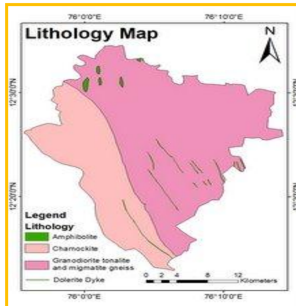
Fig. 2: Lithology of the Study area.
