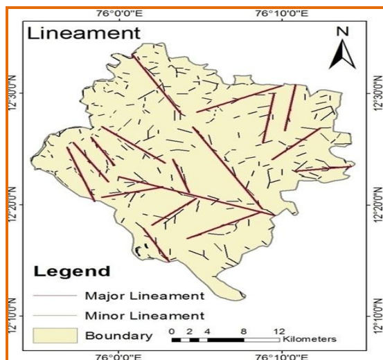
Fig. 5: lineaments of the Study area.
