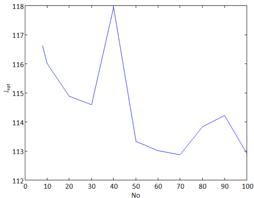
Figure 7: Discrete-time optimal average cost J_{opt} versus sampling period T_0 .
