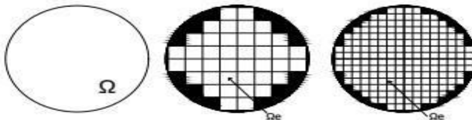
Figure 1: Mesh size of the domain \Omega_e and variation of the geometric discretization error.
