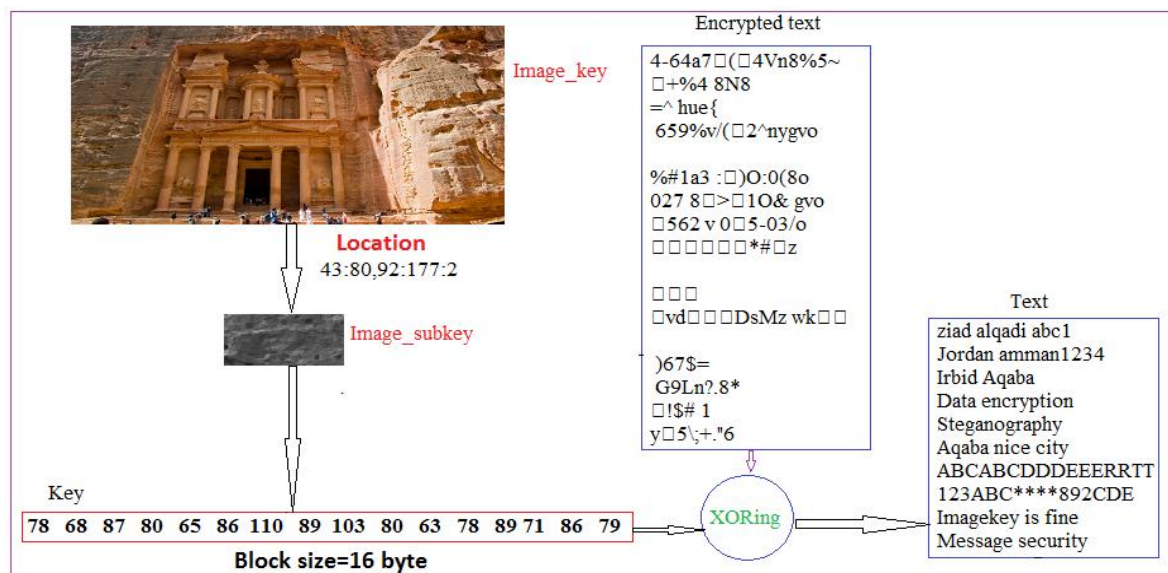
Figure 7: Blocks decryption.
