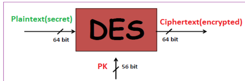
Figure 4: DES encryption.
