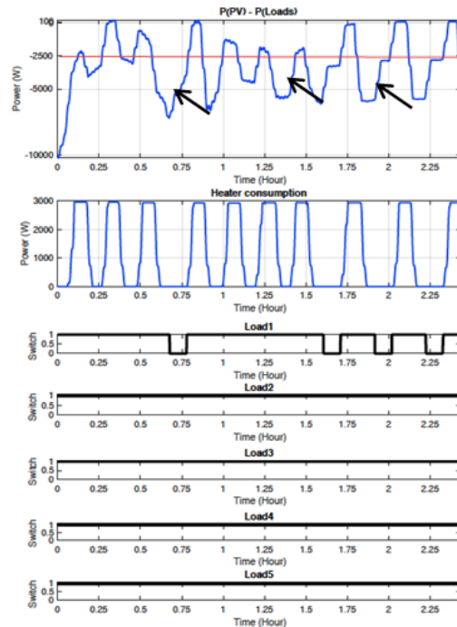
Fig.9 Simulation results at firing angle = 180^{\circ}
