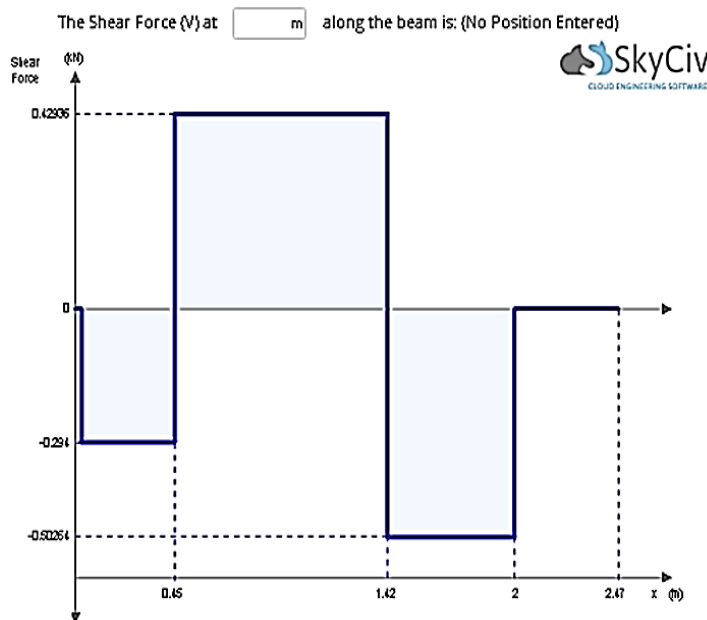
Figure 15: Shear Force Diagram (SFD) [10]
