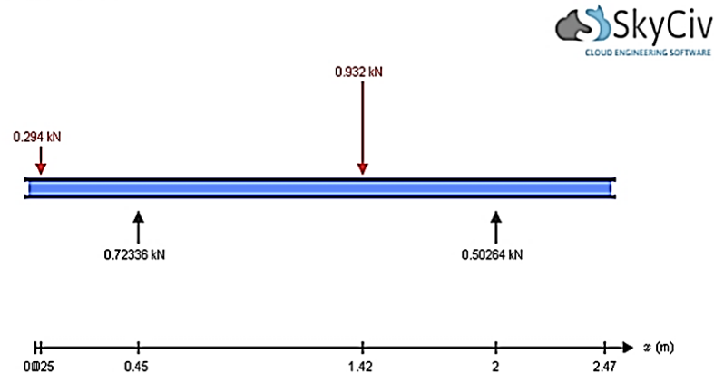
Figure 14: Free Body Diagram (FBD). [10]
