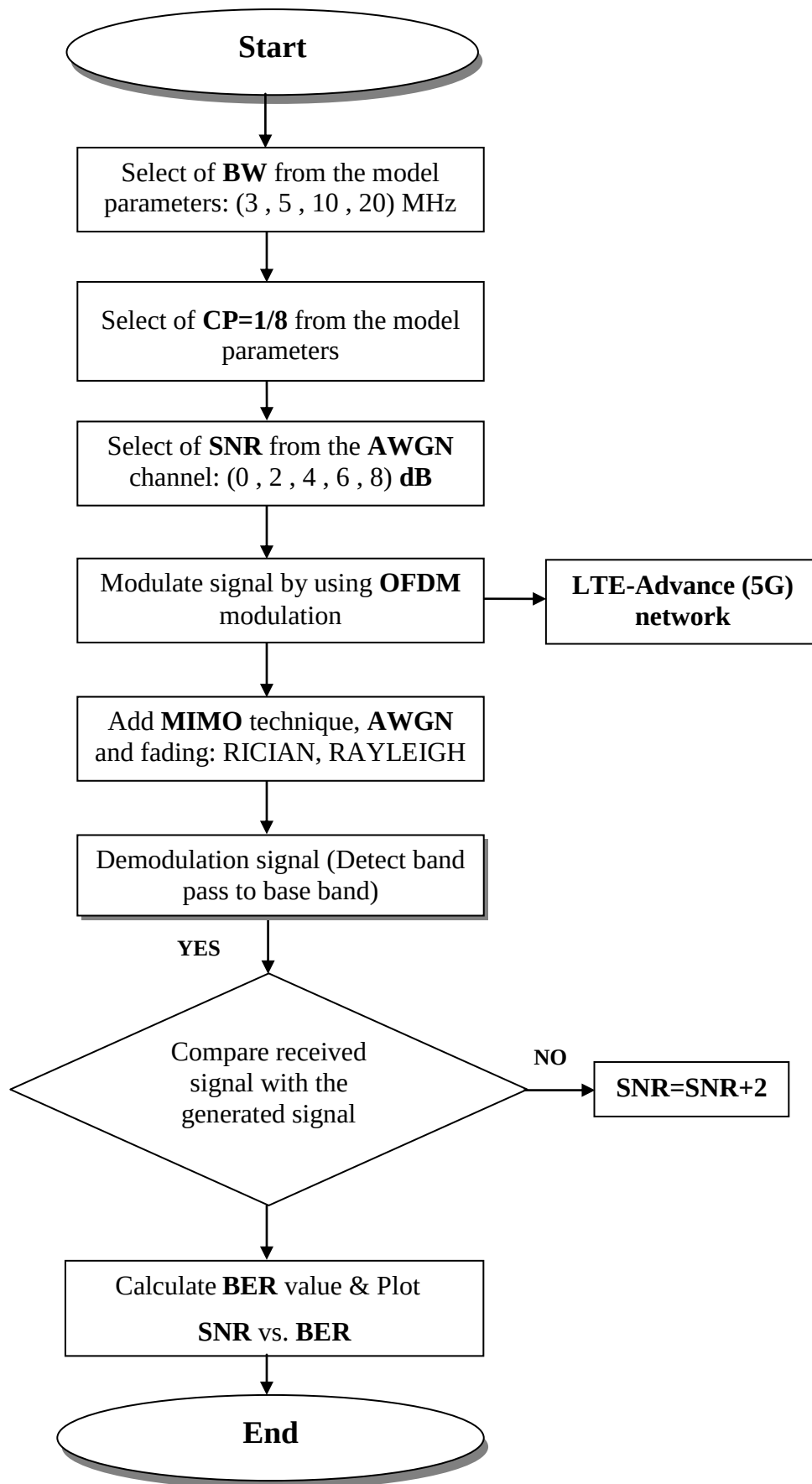
Figure 3: Computer model.
